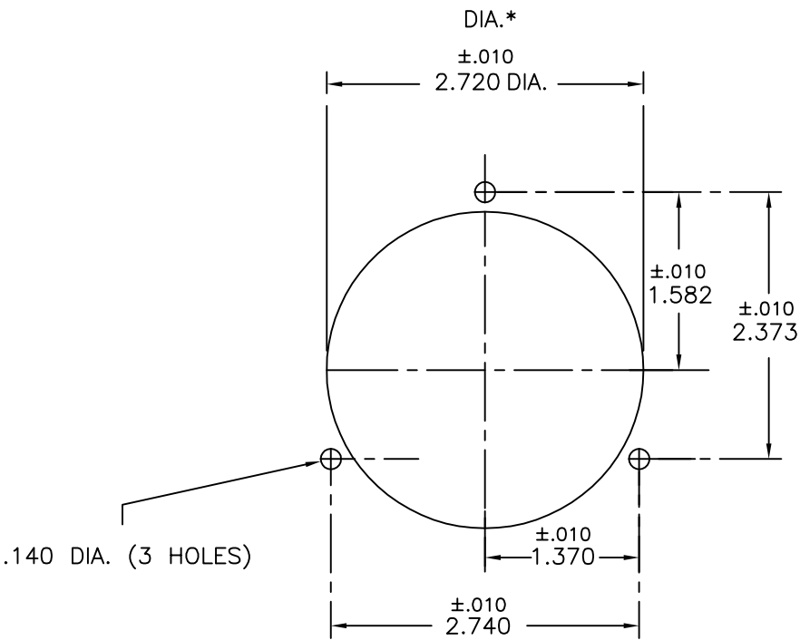
PANEL DRILLING
